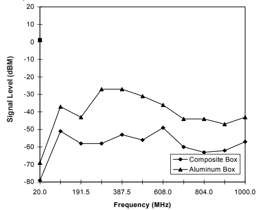
Radiated Emissions
