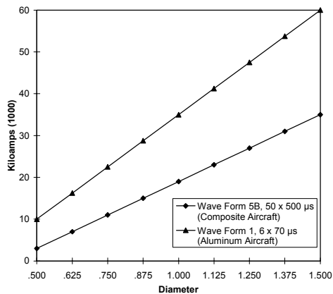
Indirect Lightning Strike Threshold SAE - AE4L-87-3, Wave Forms 1 & 5B
